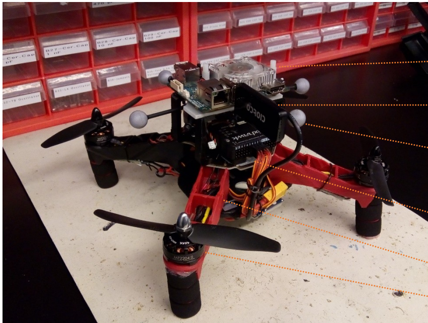
Figure 1. RISC Boot Camp UAV Platform
