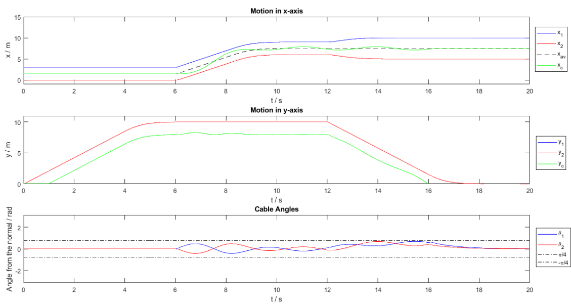
Figure 9. Evolution of System Trajectory while Performing Specified Task
