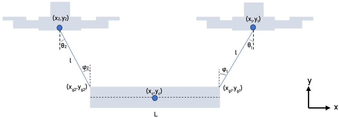
Figure 5. Simplified System Diagram: Carrying Flight Mode
