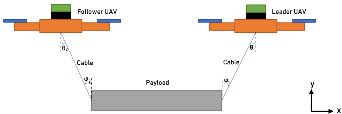
Figure 2: Proposed CPT Scheme (Side View)
